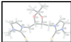
Fig. 2. View of the molecular structures of C16 molecule of showing 50% displacement ellipsoids. The H atoms are drawn as spheres of arbitrary radius.
